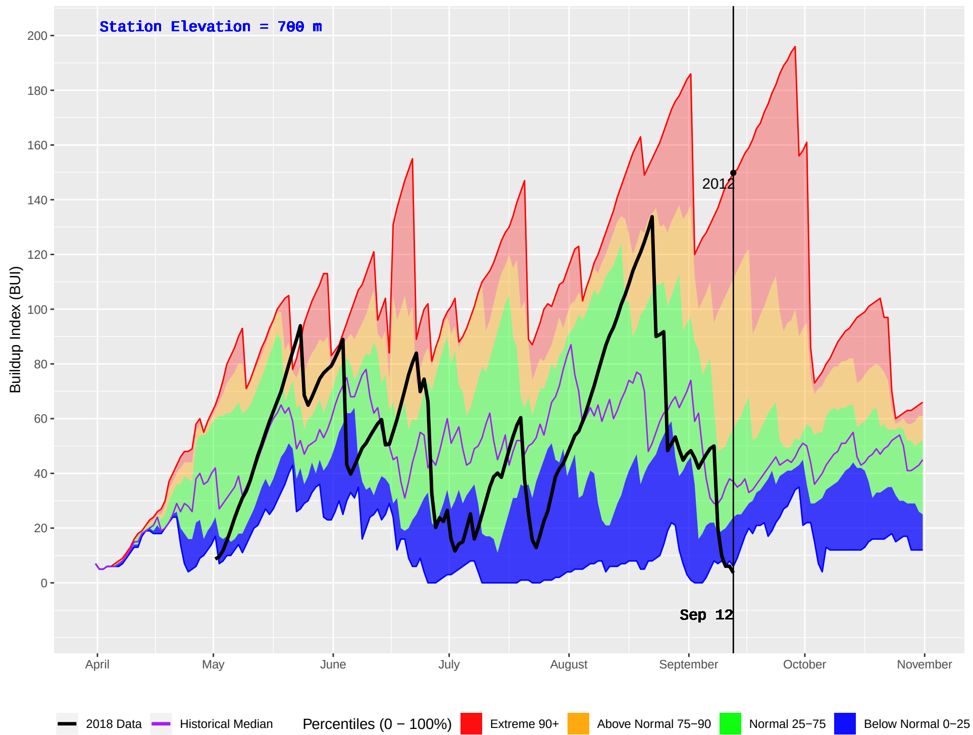
OSBORN (1045) : Historical (2009–2016) and Current (2018) Daily Buildup Index (BUI)
