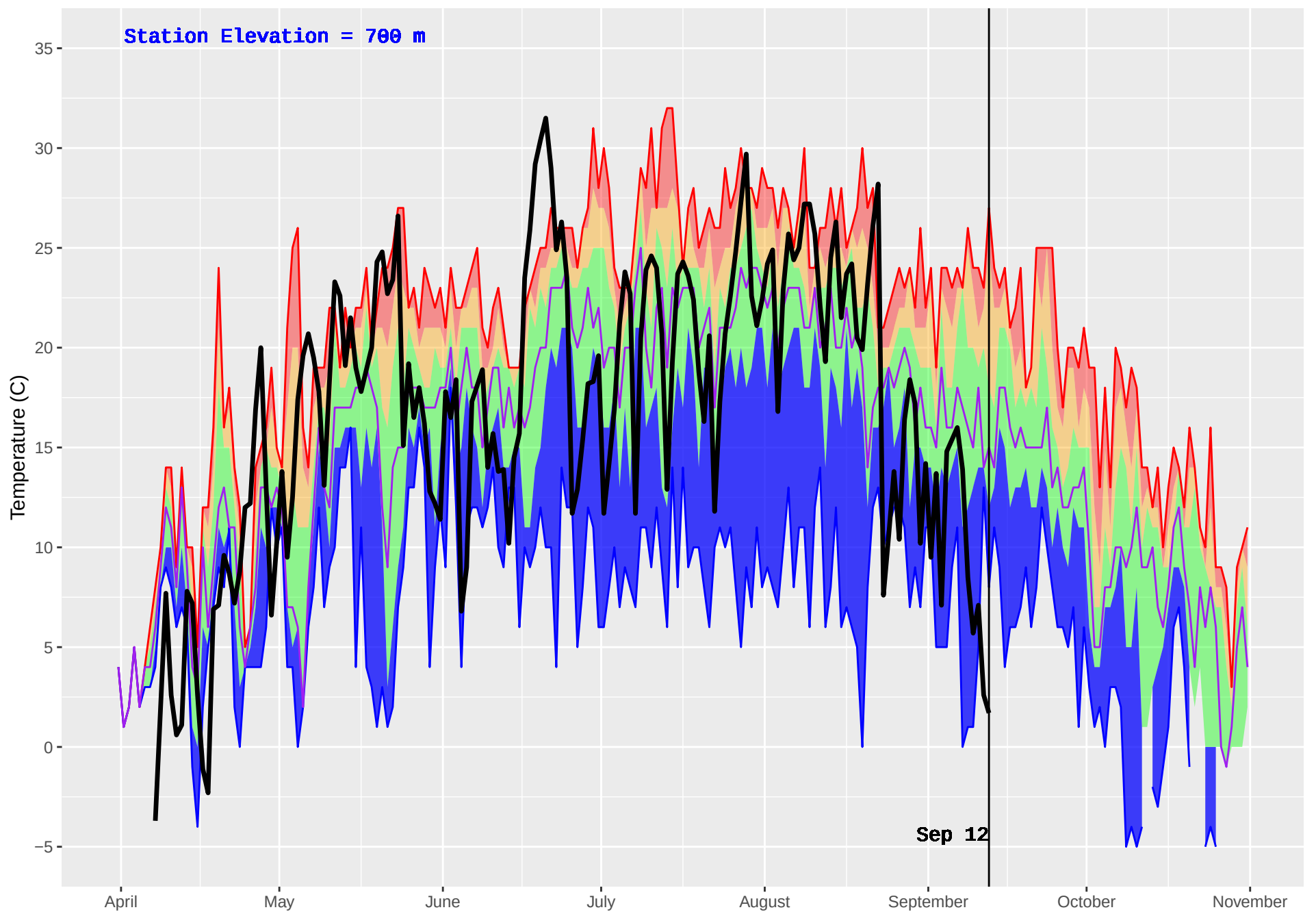
OSBORN (1045) : Historical (2009–2016) and Current (2018) Daily Temperature
